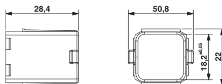
Dimensional drawing
