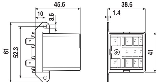
062.60 with relay
