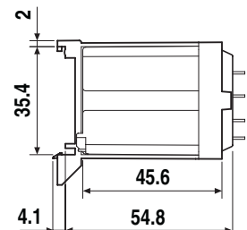
062.07 with relay
