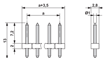
Dimensioned drawing
