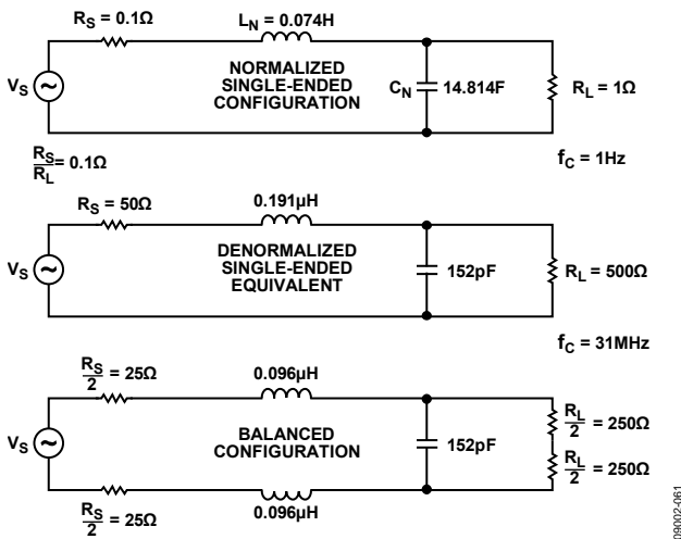
Figure 55. Second-Order Butterworth, Low-Pass Filter Design Example
