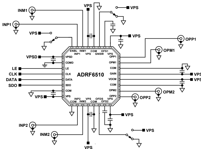
Figure 49. Basic Connections
