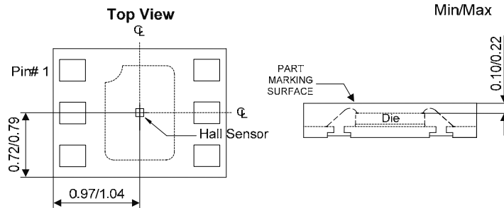
Sensor Location
