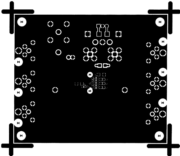
Figure 7. Circuit Side
