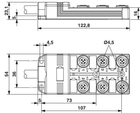
Dimensioned drawing
