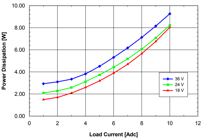
Fig. 5.0V.7: Power dissipation vs. load current and input voltage for SQ24T/S10050 converter mounted vertically with air flowing from pin 3 to pin 1 at a rate of 300 LFM (1.5 m/s) and T_a = 25^\circ\text{C} .
