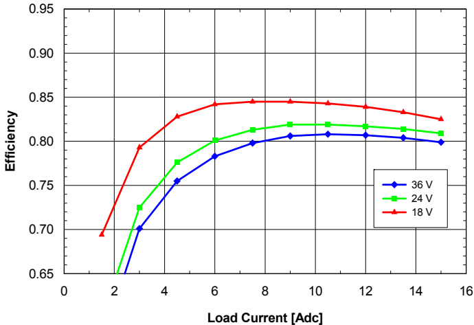
Fig. 1.2V.5: Efficiency vs. load current and input voltage for SQ24T/S15012 converter mounted vertically with air flowing from pin 3 to pin 1 at a rate of 300 LFM (1.5 m/s) and T_a = 25^\circ\text{C} .
