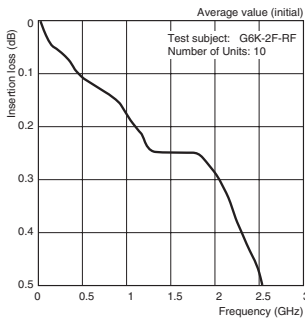
High-frequency Characteristics (Insertion Loss) (See notes 1 and 2.)
