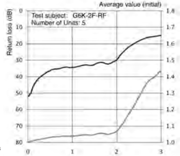
High-frequency Characteristics (Return Loss V.S.WR) (See notes 1 and 2.)
