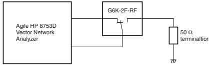
High-frequency Characteristics (Isolation) (See notes 1 and 2.)
