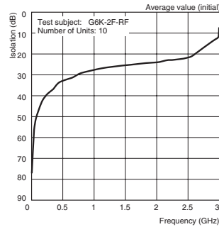
High-frequency Characteristics (Isolation) (See notes 1 and 2.)
