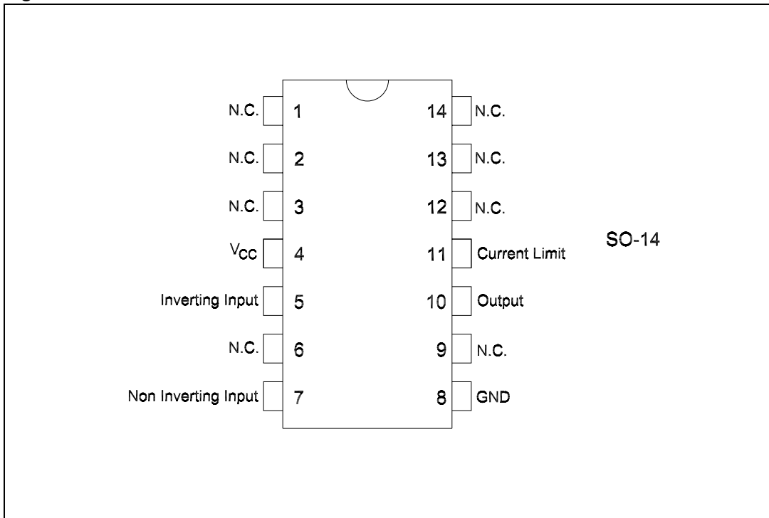
Figure 2. Pin connections
