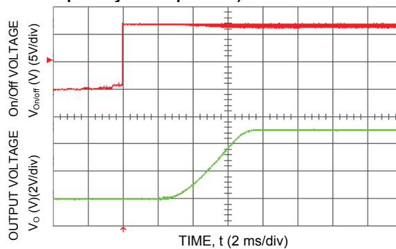
Figure 14. Typical Start-Up Using Remote On/Off ( V_{in} = 12.0 Vdc, V_o = 5.0 Vdc, I_o = 10 A).
