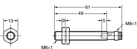
E2A-S08LS02-M5-□□
