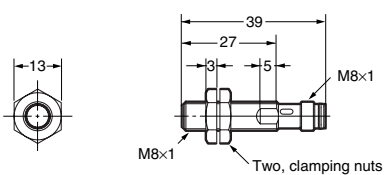
E2A-S08KS02-M5-□□
